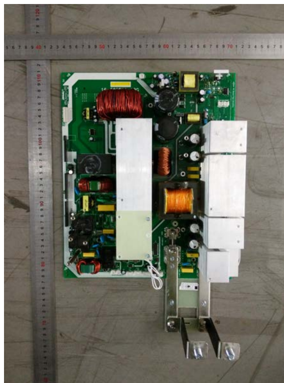
Fig. 8 -- Main power board components view
