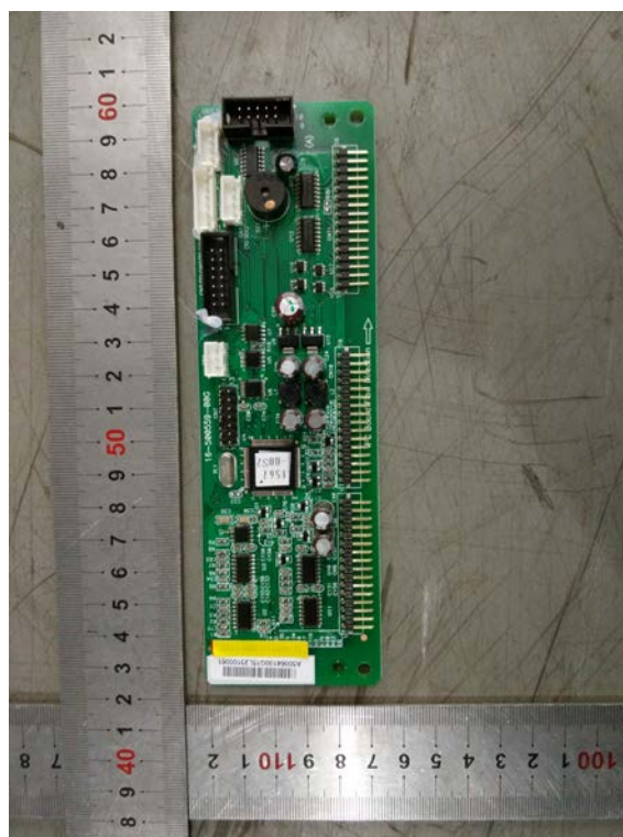
Fig. 6 -- Control board components view
