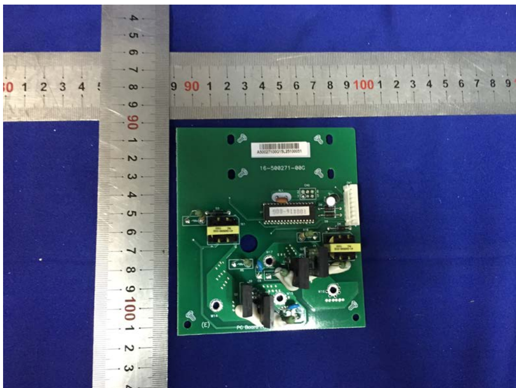
Fig. 28 -- SCR board components view
