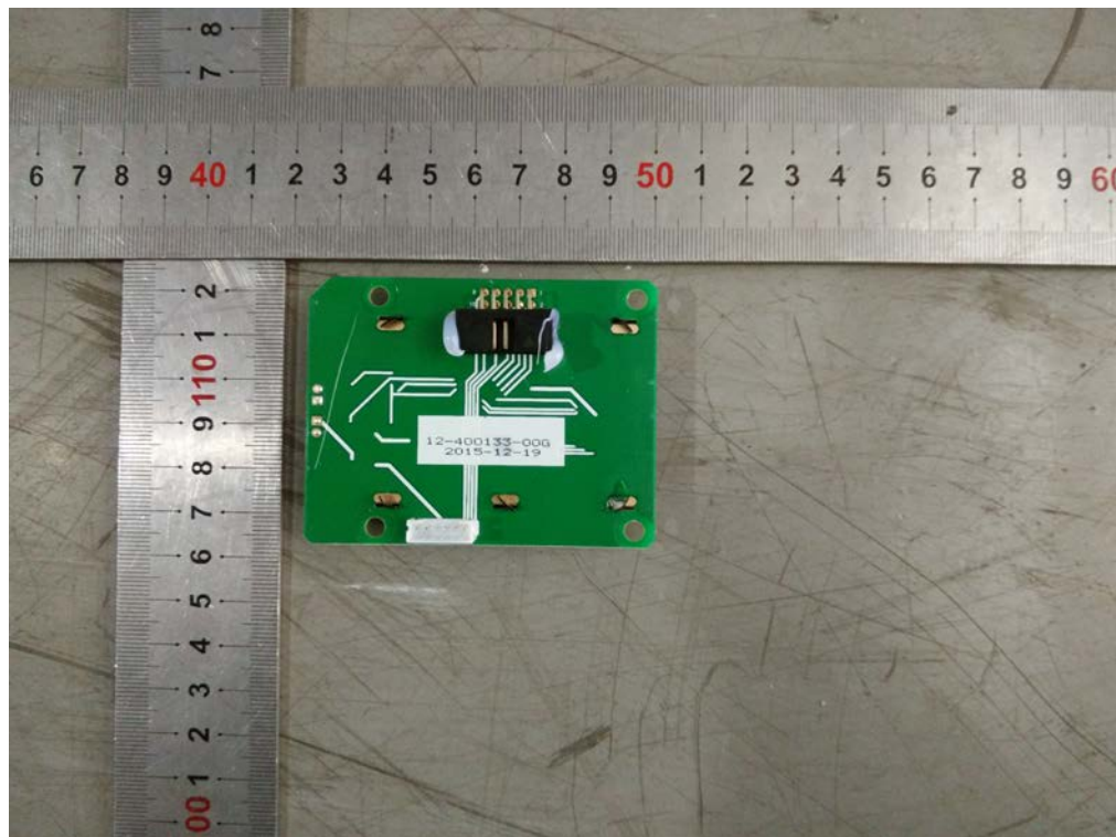
Fig. 5 -- Display board trace view
