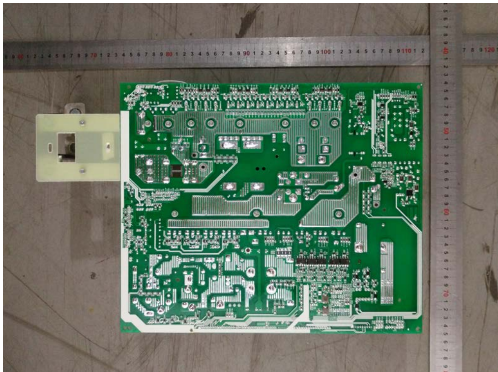
Fig. 9 -- Main power board trace view
