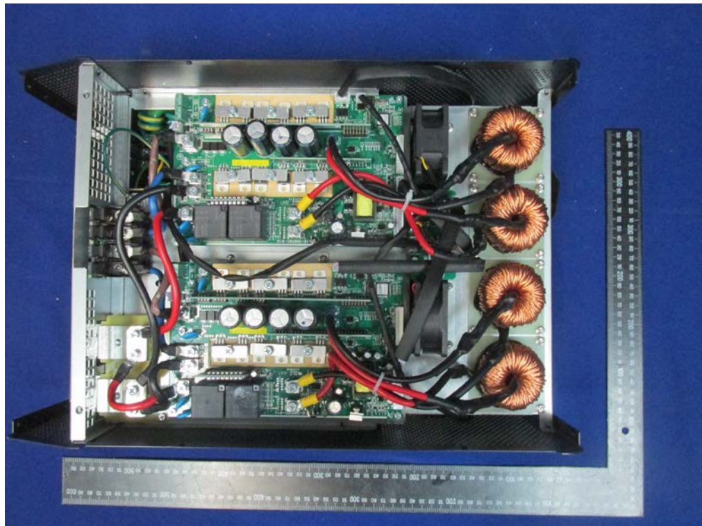
Fig. 3 -- Inside view
