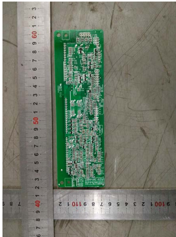
Fig. 7 -- Control board trace view
