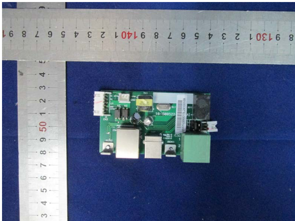
Fig. 30 -- Communication board components view
