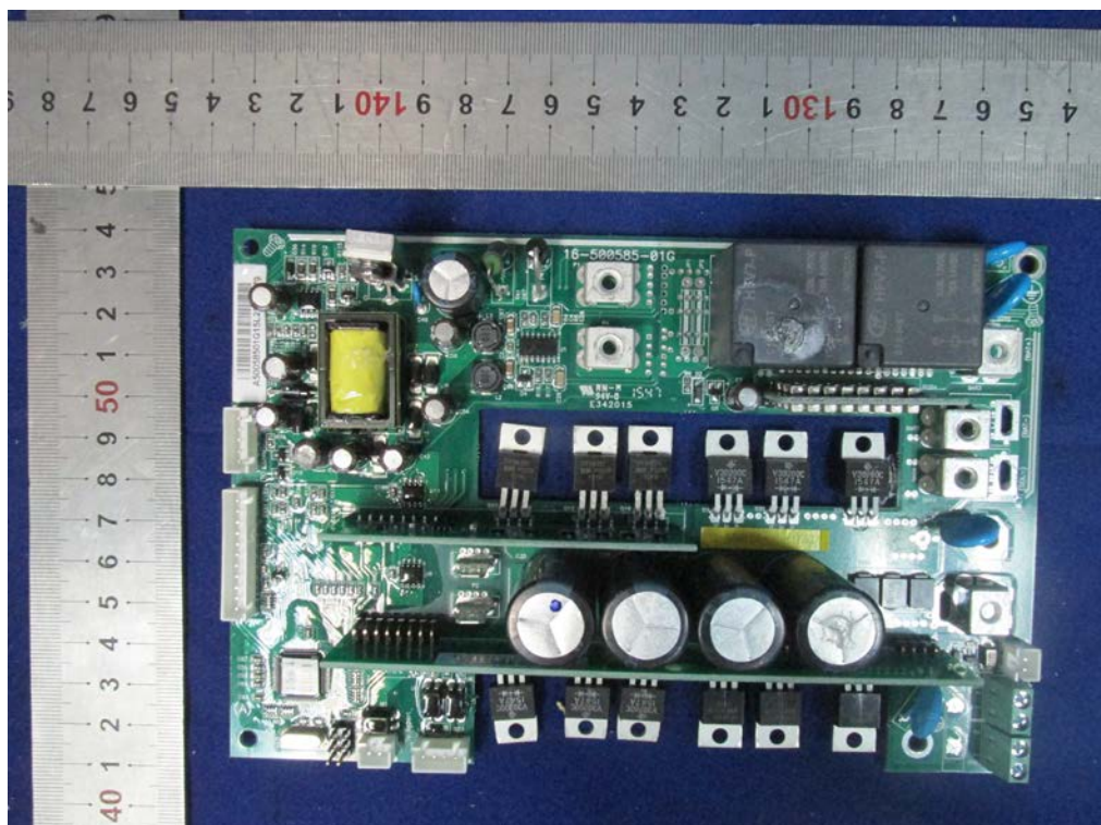
Fig. 14 -- PV board components view
