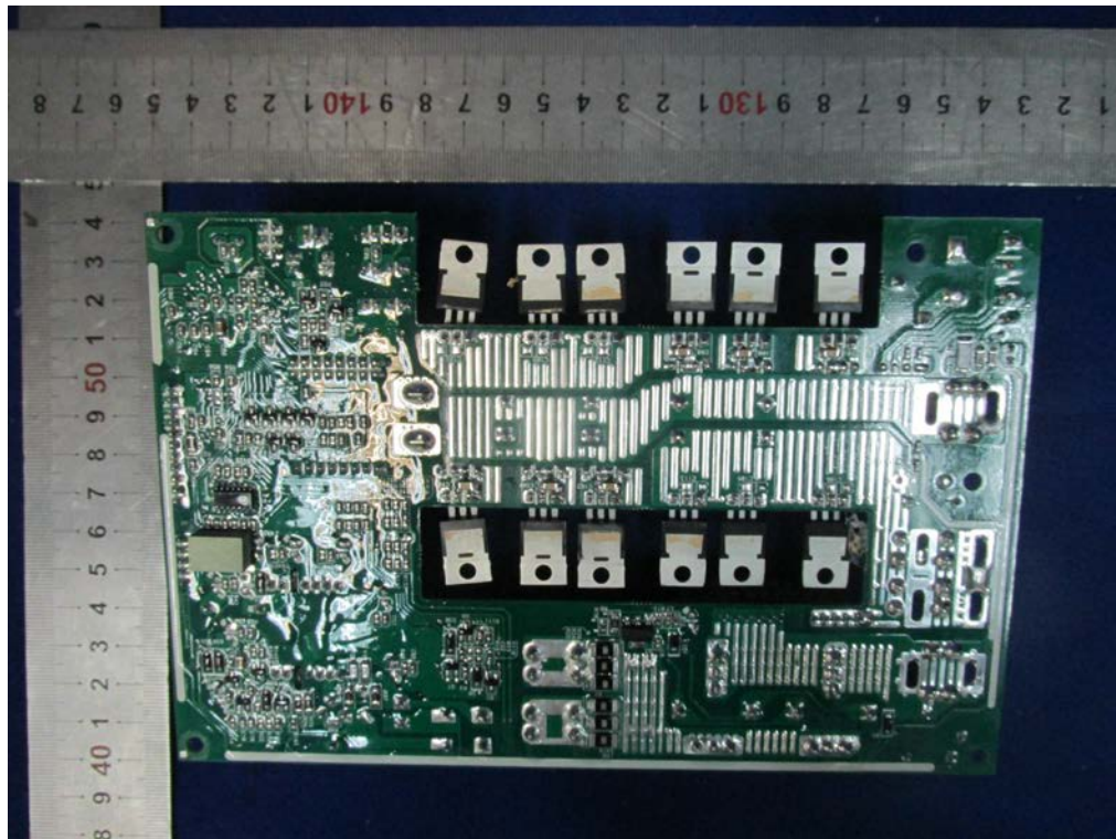
Fig. 15 -- PV board trace view
