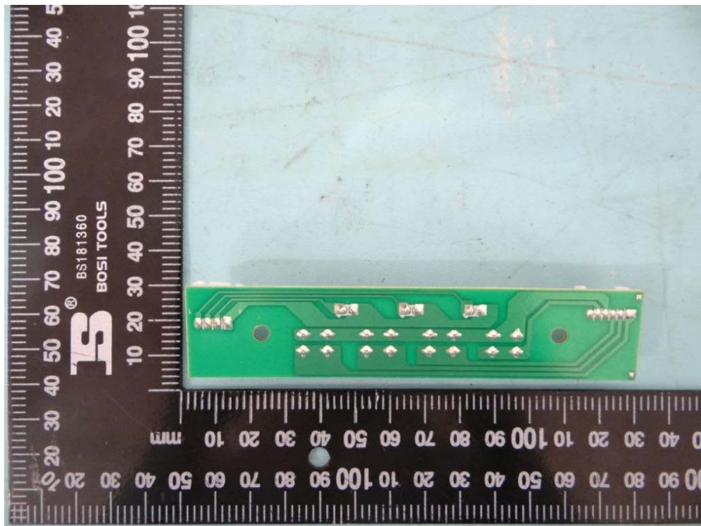
Fig. 35 -- Button board trace view
