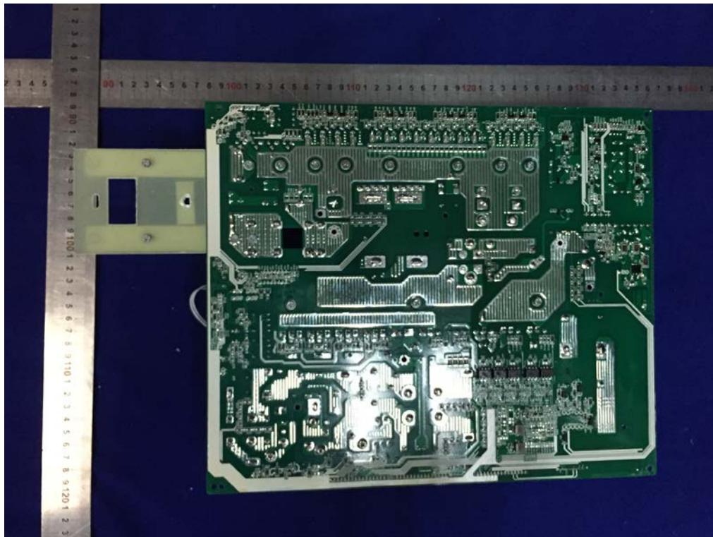
Fig. 27 -- Main power board trace view
