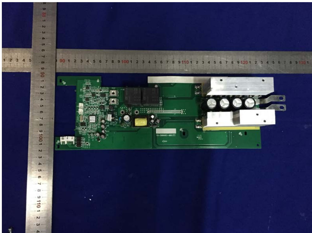
Fig. 32 -- PV board components view
