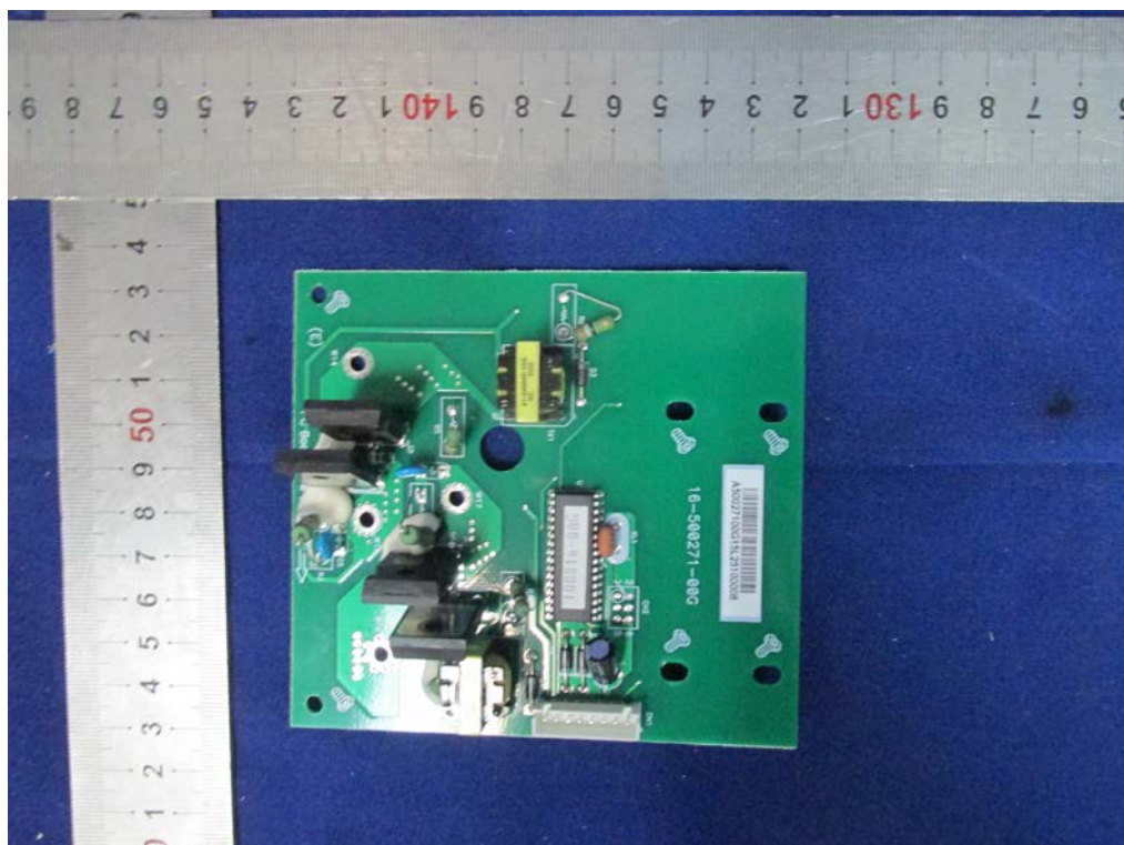
Fig. 10 -- SCR board components view
