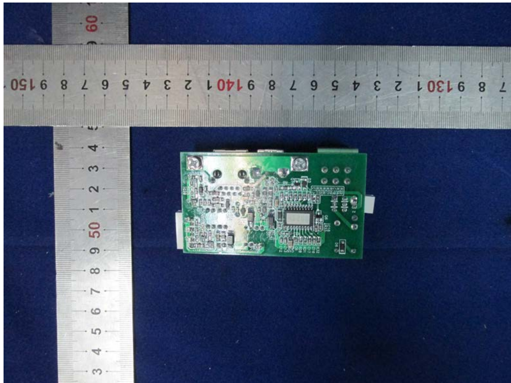
Fig. 31 -- Communication board trace view
