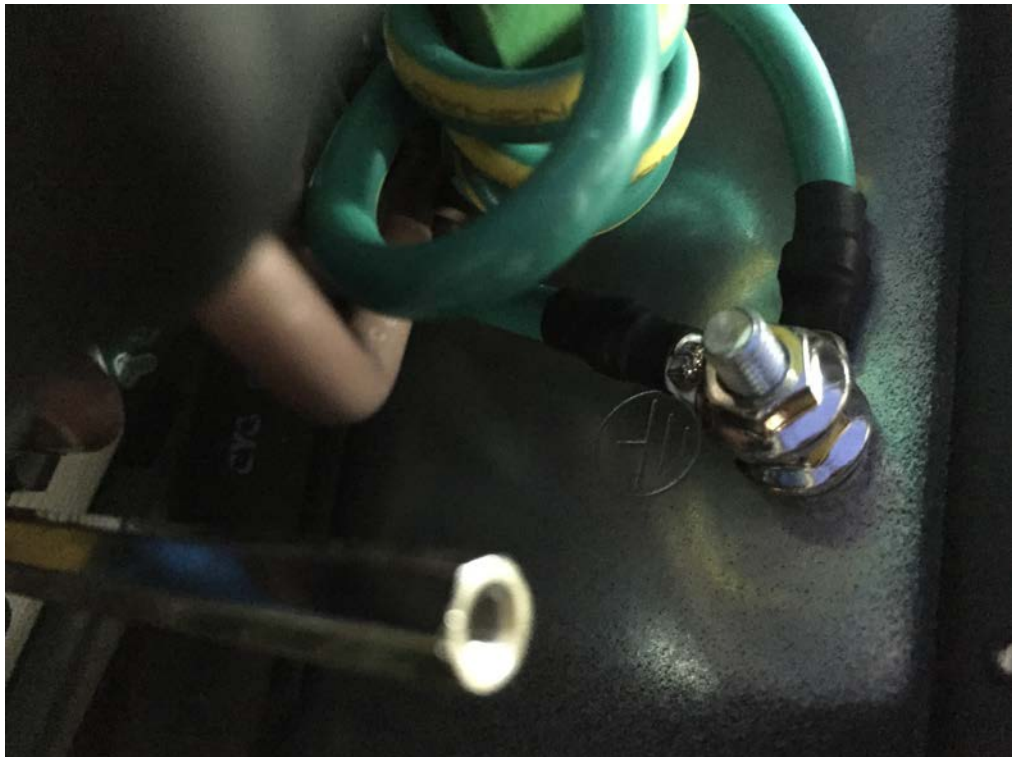
Fig. 36 -- Earth connection and earth marking
