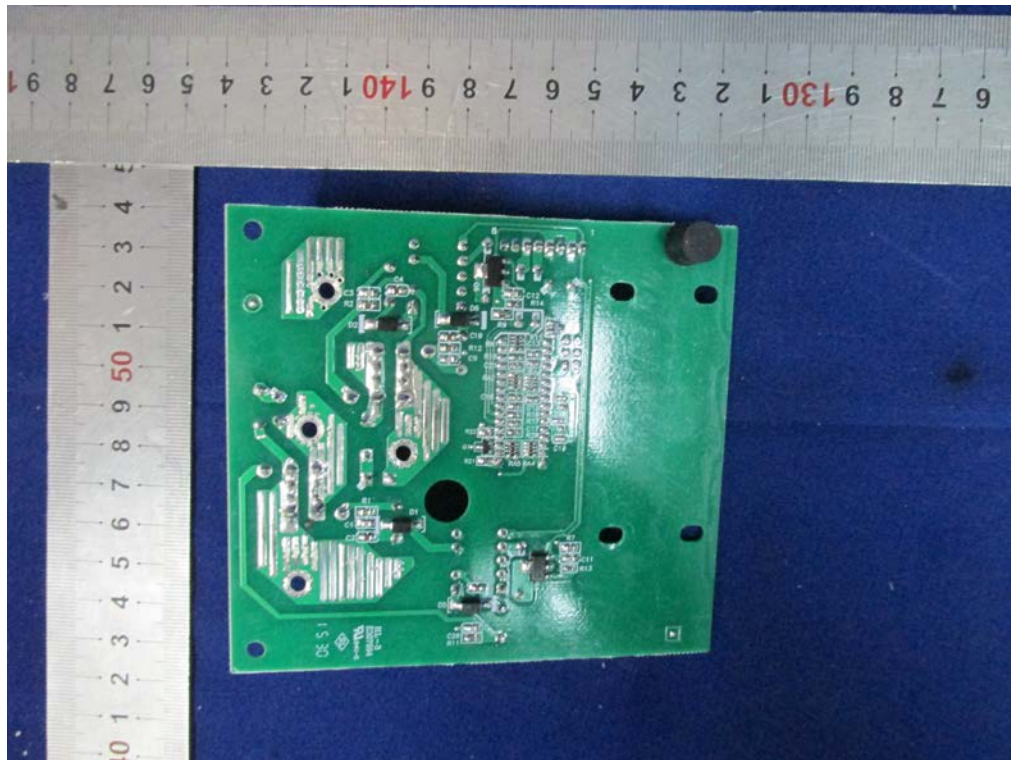
Fig. 11 -- SCR board trace view
