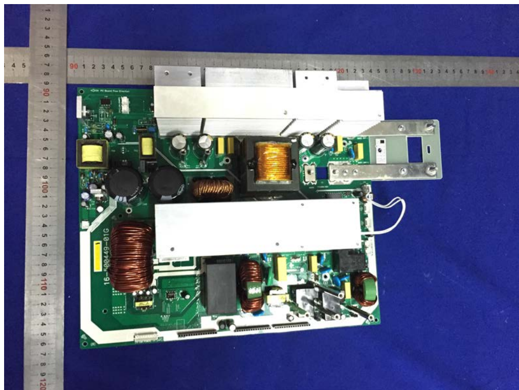
Fig. 26 -- Main power board components view
