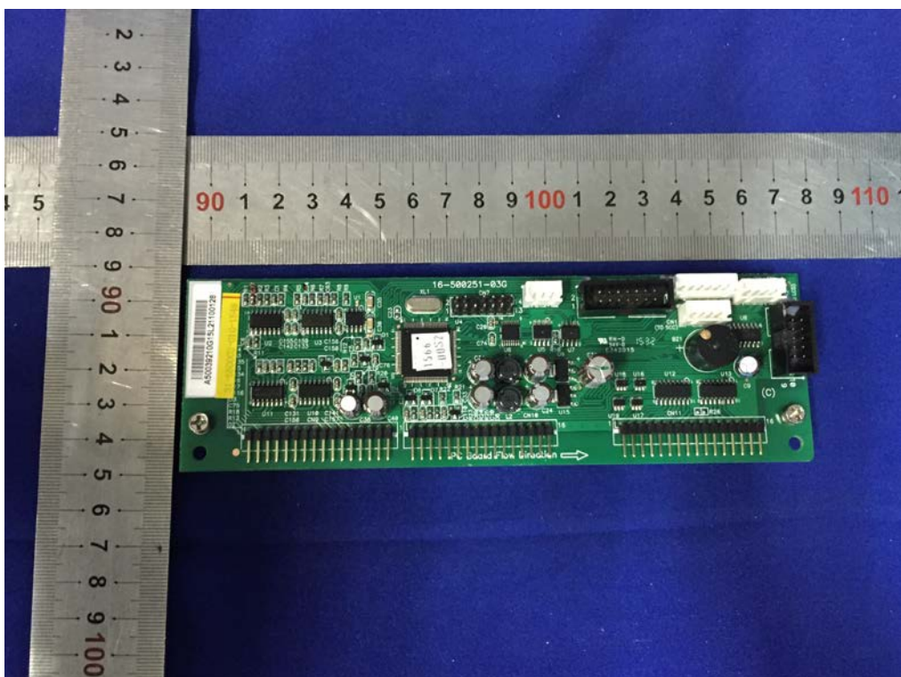
Fig. 24 -- Control board components view
