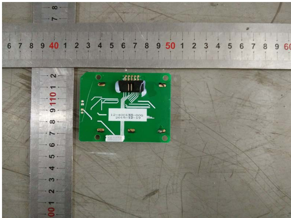
Fig. 23 -- Display board trace view
